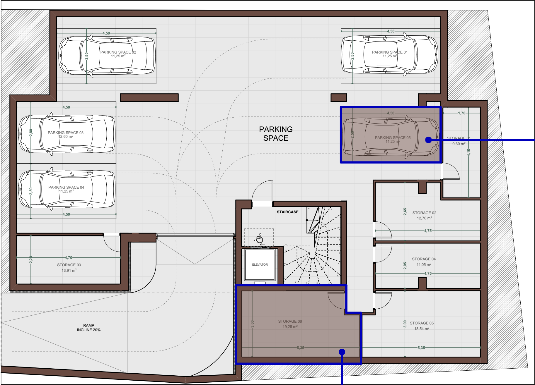
STORAGE SPACES & PARKING SPACE LEVEL -1
