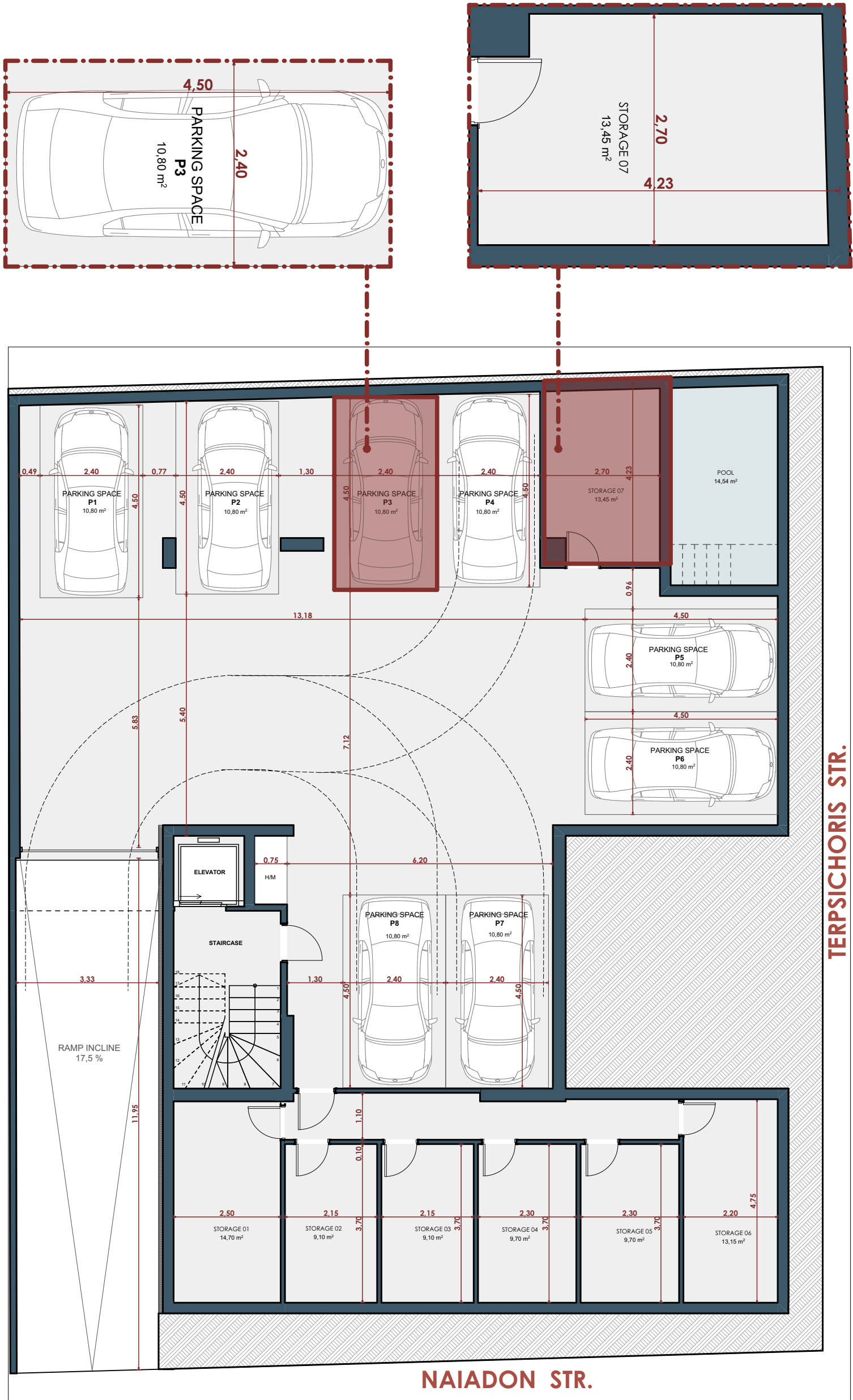
STORAGE SPACES & PARKING SPACE LEVEL -1
