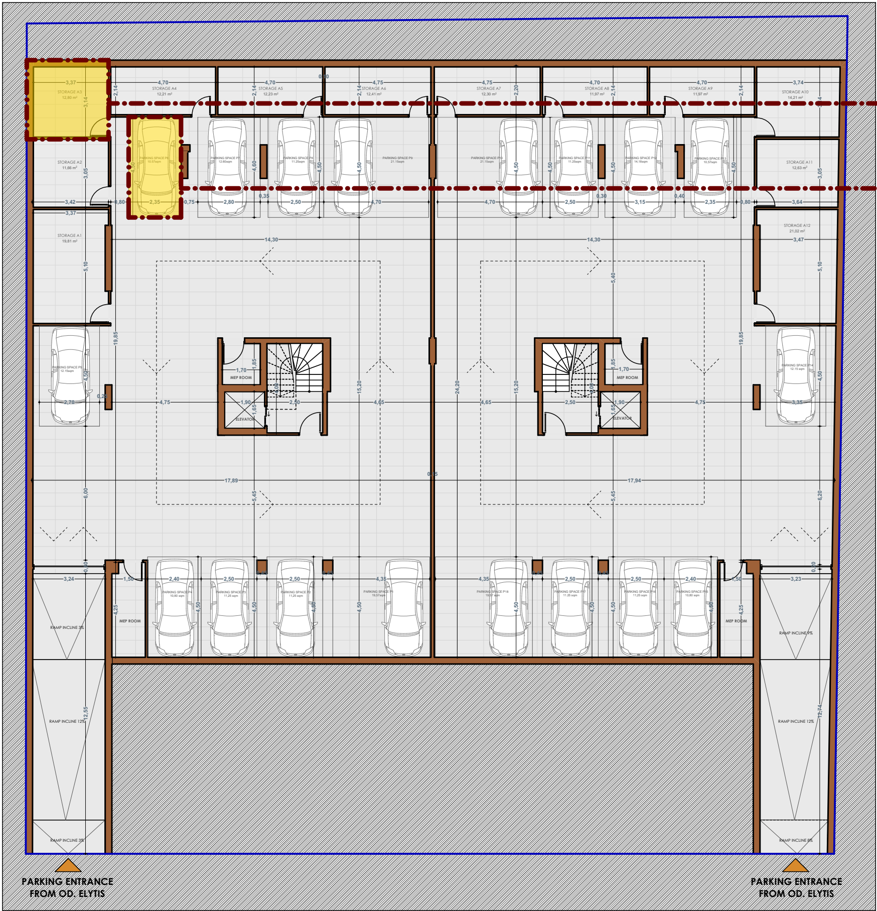
STORAGE SPACES & PARKING SPACE LEVEL -1
